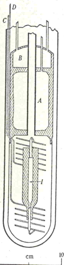
FIGURE 2. The calorimeter and cryostat.
